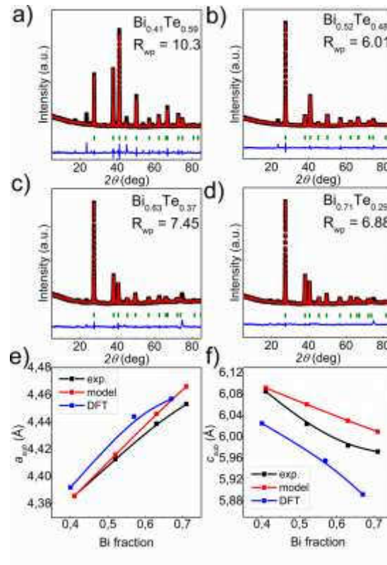
Figure 4. (a), (b), (c), (d) The results of the profile fitting with observed, calculated, and difference patterns of electrodeposited \text{Bi}_x\text{Te}_y films of different composition controlled by electrolyte composition. Dependence of the subcell parameters a_{sub} (e), and c_{sub} (f) on bismuth content in the deposited films. Red points show subcell parameters calculated for alternating \text{Bi}_2\text{Te}_3 quintuples and Bi-bilayers using stacking model[1], black points show subcell parameters determined from experimental XRD data, blue points show subcell parameters calculated using DFT.
