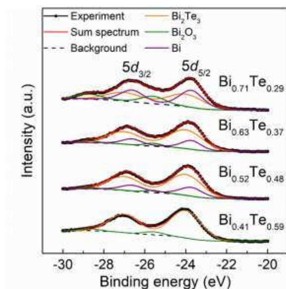
Figure 6. X-ray photoelectron spectra of (\text{Bi}_2)_m(\text{Bi}_2\text{Te}_3)_n films of various stoichiometry. Dotted line represents background line, Orange - 5d_{5/2} + 5d_{3/2} band of \text{Bi}_2\text{Te}_3 , green - 5d_{5/2} + 5d_{3/2} band of \text{Bi}_2\text{O}_3 ,
