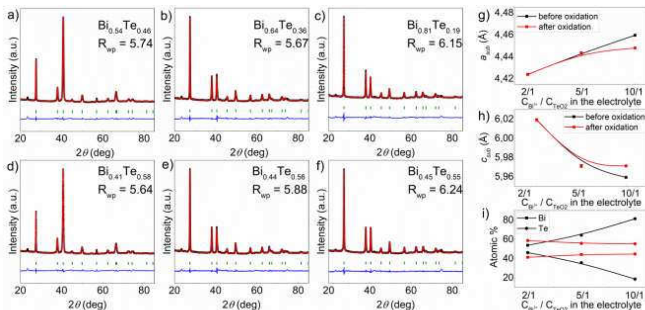
Figure 8. The results of profile fitting with observed, calculated, and difference patterns of (Bi_2)_m(Bi_2Te_3)_n films deposited from different electrolytes: c(Bi^{3+})/c(TeO_2) = 2 before oxidation (a); after oxidation (b); c(Bi^{3+})/c(TeO_2) = 5 before oxidation (c); after oxidation (d); c(Bi^{3+})/c(TeO_2) = 10 before oxidation (e); after oxidation (f). Dependence of a_{sub} , c_{sub} and films composition (g, h and i respectively) before (black lines) and after (red lines) oxidation of bismuth bilayers.
